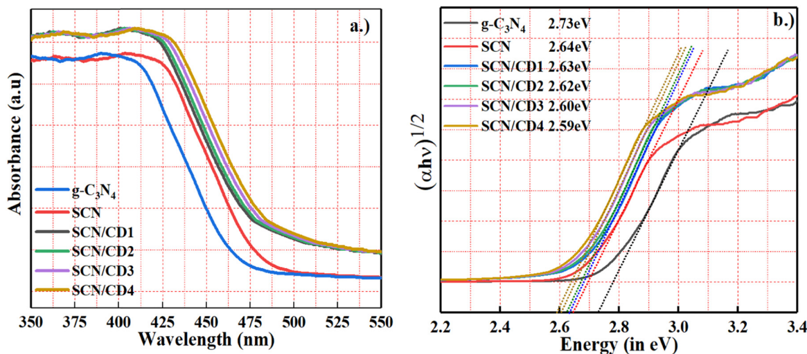
Fig. 5 (a) UV-vis diffuse reflectance of g\text{-C}_3\text{N}_4 , SCN, SCN/CD1, SCN/CD2, SCN/CD3 and SCN/CD4 (b) Tauc plot representing the bandgap energies of g\text{-C}_3\text{N}_4 , SCN, SCN/CD1, SCN/CD2, SCN/CD3 and SCN/CD4.
