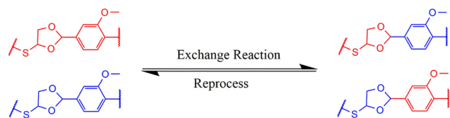
Scheme 2 Exchange reaction of VTCO-NCO.
