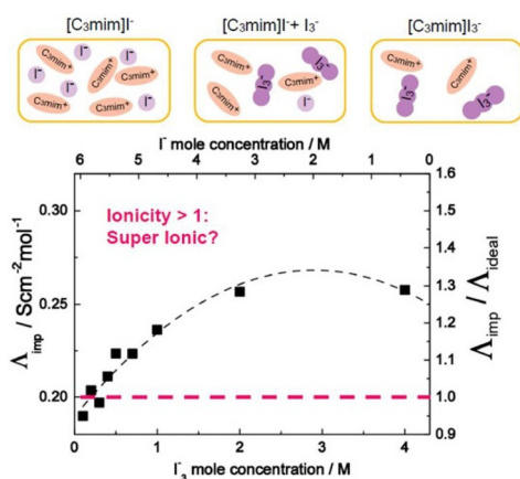
Fig. 5 Molar conductivity ( \Lambda_{\text{imp}} ) and ionicity ( \Lambda_{\text{imp}}/\Lambda_{\text{ideal}} ) of [C 3 mim] + I - with added I 2 as a function of I 3 - (I - ) concentration at iso-viscosity state of 0.2 Pa s. Reproduced from ref. 65 with permission from RSC, Copyright [2018].
