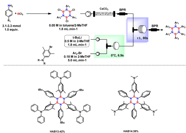
Fig. 5 Synthesis of aminated HABs under continuous flow conditions. Reaction conditions: Ar-Br (0.18 M in 2-MeTHF), t -BuLi (0.5 M in pentane/2-MeTHF), and TCB solution (0.05 M in toluene/heptane/2-MeTHF) produced from aniline derivatives (1.0 equiv.); BCl 3 (1.2 equiv.) were introduced to the flow system fabricated by PEEK Tee (ID: 0.5 mm) and PTFE tube (Øi.d.: 1 mm) using a high-pressure syringe pump.
