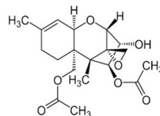
Diacetoxyscirpenol
