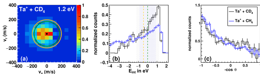
Fig. 4 Differential cross section of the reaction \text{Ta}^+ + \text{CD}_4 at 1.2 eV (a). Kinematic cut-offs (green: {}^5\text{Ta}^+ ; orange: {}^3\text{Ta}^+ are superimposed and calculated using the exothermicities given in Fig. 1. (b) Integrated internal energy distributions for the reaction with \text{CD}_4 in black and \text{CH}_4 in blue together with the \pm 1\sigma -error illustrated as a shaded area around the kinematic cut-off of the ground-state reaction ( \text{CD}_4 in blue and \text{CH}_4 in grey), which is given as the vertical line (green). The \pm 1\sigma -error is derived from Gaussian error propagation of the energy and angular spread of the reactant beams. 54 (c) The integrated angular distribution for the reaction with \text{CD}_4 in black and \text{CH}_4 in blue.
