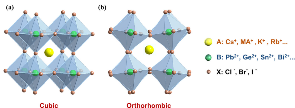
Fig. 3 (a) Cubic and (b) orthorhombic crystal structures of 3D ABX 3 perovskites.
