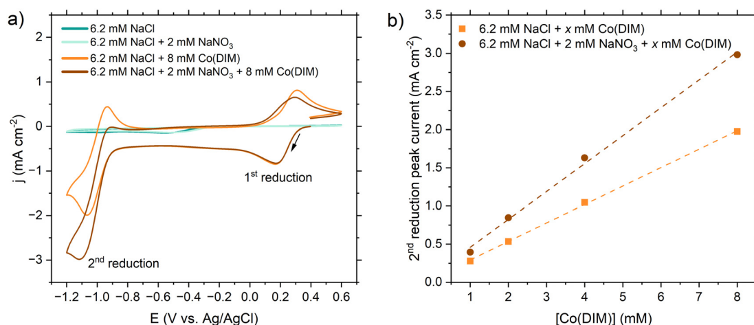
Fig. 1 (a) Cyclic voltammograms collected in 6.2 mM NaCl (background electrolyte matching the Cl − concentration in real wastewater), 6.2 mM NaCl with 2 mM NaNO 3 (background electrolyte with representative nitrate concentration), 6.2 mM NaCl with 8 mM Co(DIM) (background electrolyte with catalyst), and 6.2 mM NaCl with 2 mM NaNO 3 and 8 mM Co(DIM) (background electrolyte with catalyst and representative nitrate concentrations). Working electrode: 5 mm GC disk. Counter electrode: 6.4 mm graphite rod. Reference electrode: Ag/AgCl (4.0 M KCl). Scan rate: 100 mV s −1 . (b) Peak current density of the second reduction peak ( \sim -1.1 V vs. Ag/AgCl) of 6.2 mM NaCl with 8 mM Co(DIM) in the presence and absence of 2 mM NaNO 3 . Associated voltammograms are provided in Fig. S4 (ESI†). The excess factor, defined as the concentration of substrate (NO 3 − ) divided by the concentration of catalyst (Co(DIM)), ranged from 2 to 200 previously. To address dilute real wastewaters, we minimized the excess factor with 8 mM Co(DIM) (the observed solubility limit at room temperature) to maximize NO 3 RR activity (excess factor = 0.25, Fig. 1b).
