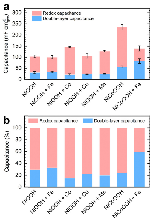
Fig. 3 (a) Capacitance contributions of NF–NiOOH electrodes after GCD conditioning in purified 1 M KOH electrolyte spiked with transition metal cations (100 ppb M n+ ); (b) relative contribution of each type of capacitance ( C_{redox} and C_{dl} ) to the total capacitance ( C_{tot} ).
