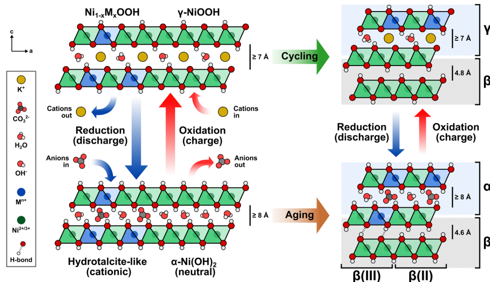
Fig. 7 Transition metal incorporation induces structural transformations of layered \text{Ni}(\text{OH})_2/\text{NiOOH} to an interstratified structure. The hydratalcite-like structure evolves into a mixed \alpha/\beta phase composition upon aging and a mixed \gamma/\beta phase composition upon electrochemical cycling/conditioning.
