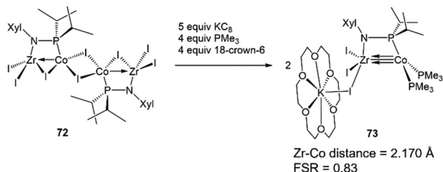
Scheme 18 Synthesis of a mono(phosphinoamide)-supported \text{Zr}^{\text{IV}}/\text{Co}^{-\text{I}} complex.
