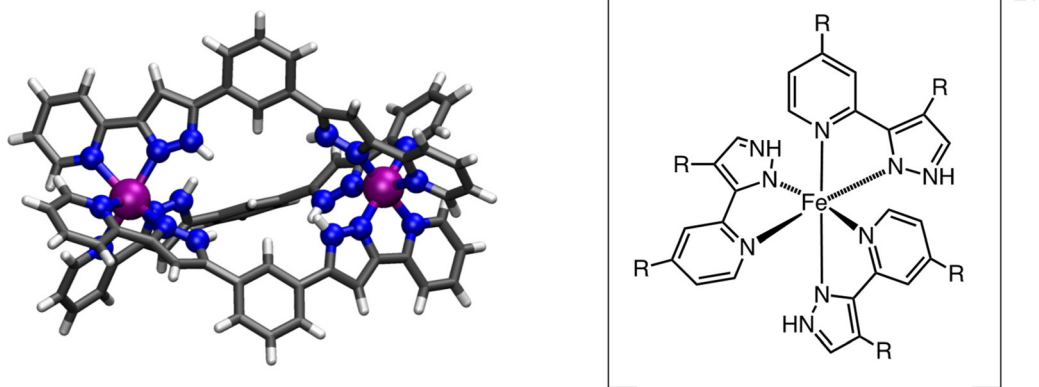
Fig. 1 (Left) The [\text{Fe}_2(\text{L}_1)_3]^{4+} system ( \text{L}_1 = 1,3\text{-bis}(3\text{-(pyridin-2-yl)-1H-pyrazol-5-yl})\text{benzene} ) and (right) schematic depiction of the subunit [\text{Fe}(\text{L}_2^{\text{R}})_3]^{2+} ( \text{L}_2 = 3\text{-(2-pyridyl)pyrazole} ), showing the R positions used to screen for ligand functionalization. Blue for N, purple for Fe, grey for C and white for H.
