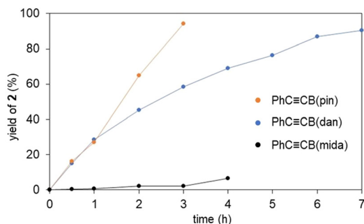
Fig. 5 Time course studies on the formation of vinylidene complexes. Reactions were performed at room temperature in CDCl 3 using an NMR tube. Yields of complexes 2 were determined by 1 H NMR spectroscopy.
