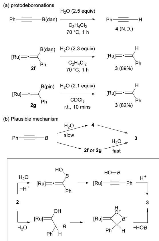
Fig. 4 (a) Control experiments and (b) a proposed reaction mechanism for the protodeboronation ([Ru] = [Ru(dppe)Cp] + ).
