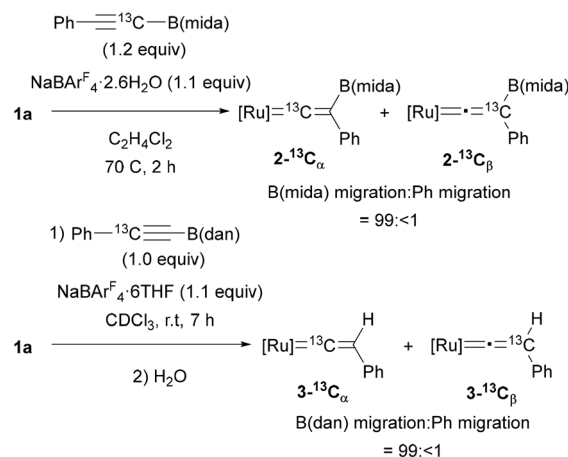
Fig. 6 Isotopic labeling experiments ([Ru] = Ru(dppe)Cp + ).
