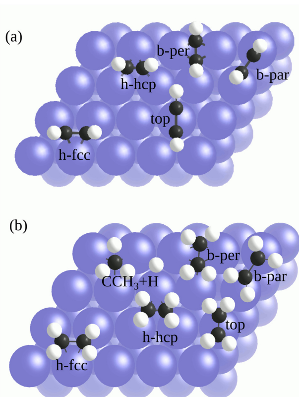
Fig. 1 Different adsorption sites for (a) \text{C}_2\text{H}_2 and (b) \text{C}_2\text{H}_4 on a fcc(111) metal surface. The \text{CCH}_3 + \text{H} in (b) shows the adsorption structure of \text{C}_2\text{H}_4 in dissociative mode. Here, \text{CCH}_3 and \text{H} adsorb at neighbouring h-fcc sites. Metal, carbon, and hydrogen atoms are shown as purple, black, and white spheres, respectively.
