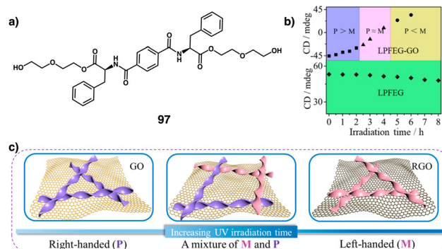
Fig. 43 (a) Structure of monomer 97 . (b) Plot of CD intensity of LPFEG and LPFEG-GO hydrogels at around 270 nm versus UV irradiation time. (c) The representative transition stages from right-handed nanofibers to left-handed twists with increasing UV irradiation time. Reproduced from ref. 238 with permission from the American Chemical Society, copyright 2020.
