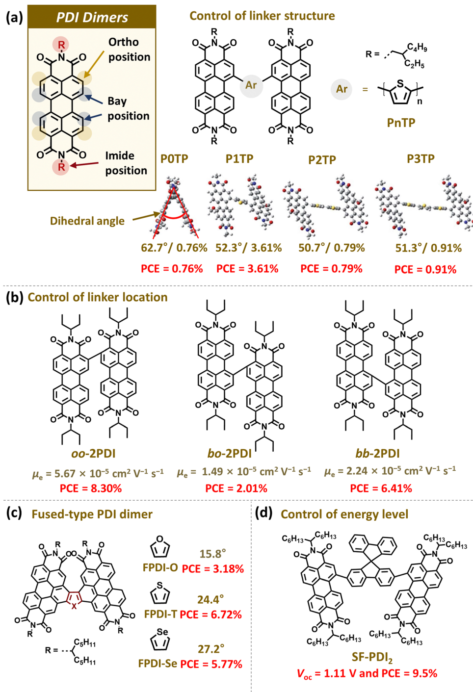
Fig. 5 Representative examples of PDI-based dimer acceptors; (a) P0TP, P1TP, P2TP, and P3TP, (b) oo-2PDI, bo-2PDI, and bb-2PDI, (c) FPDl-O, FPDl-T, and FPDl-Se, and (d) SF-PDI 2 . Reproduced from ref. 121 with permission from the Royal Society of Chemistry, copyright 2024.
