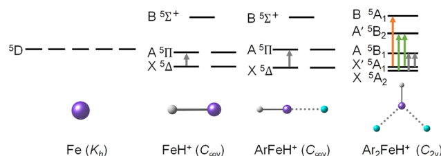
Scheme 1 Splitting of the ^5\text{D} term in iron upon addition of H ^+ and complexation with Ar. Symmetry allowed transitions from the lowest-lying states are shown with arrows. Spin–orbit coupling is not shown for clarity.
