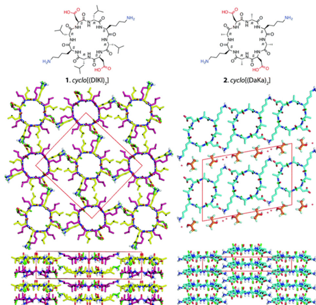
Fig. 5 Chemical structures of \text{cyclo}(\text{L-Asp-D-Leu-L-Lys-D-Leu})_2 and \text{cyclo}(\text{L-Asp-D-Ala-L-Lys-D-Ala})_2 and crystal structures of their PNTs. Reproduced with permission from ref. 34 Copyright 2017, The Royal Society of Chemistry.
