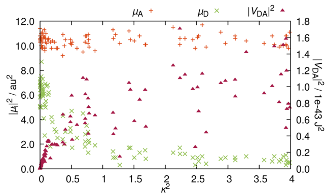
Fig. 5 Influence of the RET orientation factor \kappa^2 on the TDM strengths |\vec{\mu}_A|^2 and |\vec{\mu}_D|^2 as well as on the electrostatic interaction factor |V_{DA}|^2 for the 100 structures representative of the thermal ensemble.
