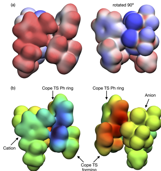
Fig. 13 Reaction B TS-[C 4 C 1 C 1 im][NTf 2 ] (a) electrostatic potential (ESP) mapped onto the 0.007 density iso-surface, red positive, blue negative, maximum \pm 0.05 a.u., (b) \Delta\rho = \text{ESP}_{\text{cluster}} - (\text{ESP}_{\text{TS}} + \text{ESP}_{\text{solvent}}) mapped onto the 0.007 a.u. ( e/a_0^3 ) density iso-surface. "Rainbow" colour scheme, blue = negative, green = neutral, red = positive, maximum \pm 0.02 a.u.
