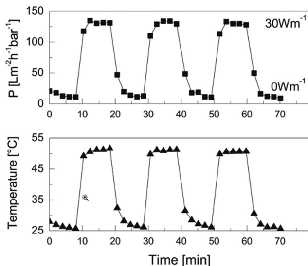
Fig. 6 The dead-end permeability ( P ) through a Si-C membrane with PVCL microgel coating was measured with heating cycles of 10 min with 30\text{Wm}^{-1} of applied power. The permeability is increased due to the collapse of the microgel. Reproduced with permission from T. Lohaus, P. de Wit, M. Kather, D. Menne, N.E. Benes, A. Pich and M. Wessling, J. Membr. Sci. , 2017, 539 , 451.
