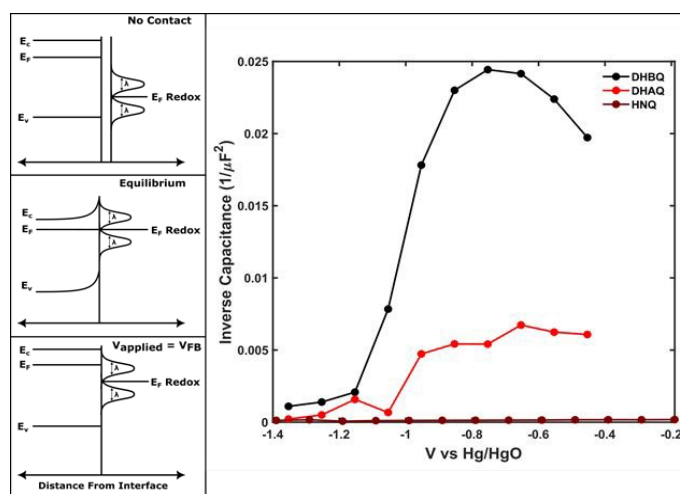
Figure 2. Semiconducting electrode-electrolyte interface, and the basis for the Mott-Schottky analysis. Upon contact, the semiconductor and electrolyte equilibrate in electron energies, and only at the flat band potential are returned to the equilibrium band structure in the solid. This flat band potential ( V_{FB} ) is quantitatively the x-intercept of the inverse capacitance with applied bias.
