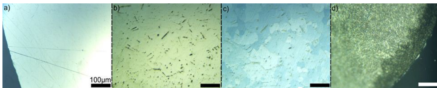
Figure 3. Optical microscopy shows different stages in Zn electrode morphology evolution. Clockwise, (a), the surface is mechanically polished, but retains micron-scale scratches/mechanical inclusions. Upon brief (ca. 1 h) exposure to alkaline electrolyte (1 M KOH, with or without mediator) the surface layer is microscopically etched (b), revealing more subsurface features. Upon imaging in crossed polarizers (at the same time), (c), the underlying grain structure is revealed. Finally, upon extended (ca. 24 h) exposure to alkaline electrolyte, the surface is covered in a non-metallic layer of corrosion products.
