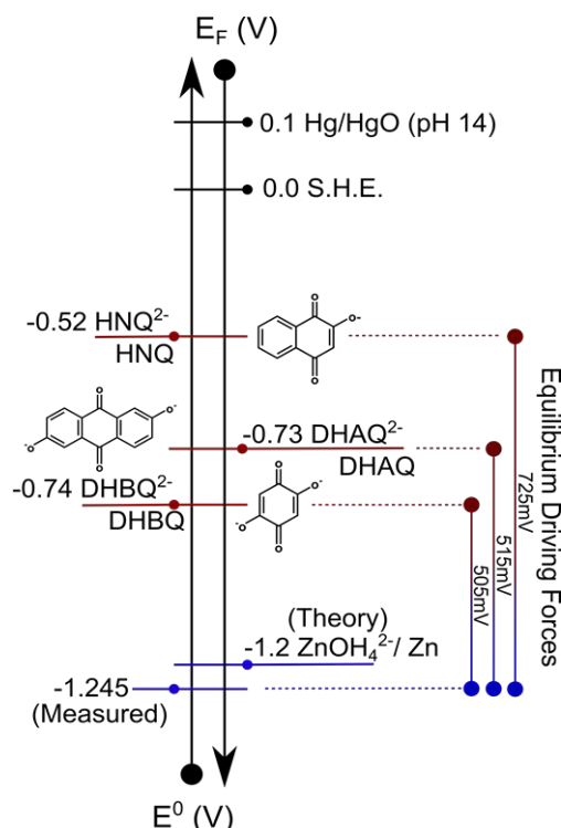
Figure 1. Electrode potential scale showing the location of the approximate redox potentials both versus a standard reference ( E^0 ) and absolute electron energy ( E_F ), for both the zinc/zincate couple and quinone redox couples selected as mediators. Equilibrium overpotentials between the liquid/solid components are indicated on the right-hand side. Please see supplementary information for complete compound names and discussion of reactions.
