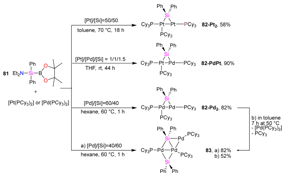
Scheme 28 Preparation of di- and trinuclear \text{Pd}(0)/\text{Pt}(0) complexes with bridging silylene ligands.
