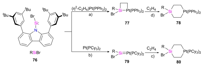
Scheme 26 Synthesis of compounds 77–80 starting from RSiBr 76 . Reaction condition: (a) toluene, RT, 12 h; (b) toluene, RT, sonication 15 min; (c) toluene, 1 atm \text{C}_2\text{H}_4 , RT, 12 h; (d) \text{C}_6\text{D}_6 , 1 atm \text{C}_2\text{H}_4 , 80 °C, 72 h.
