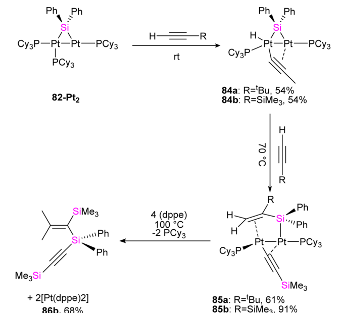
Scheme 29 The stoichiometric reaction of 82-Pt 2 with terminal alkynes.
