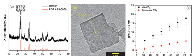
Fig. 12 (Left) X-ray diffraction data and (centre) TEM imaging of the obtained microwave synthesized \text{WO}_3 ; (Right) concentration of benzaldehyde, oxidation product of benzyl alcohol, over time during \text{WO}_3 photocatalysis. Black squares: microwave synthesized nanoplatelets; Red circles: commercial material. Credit: K. D. McDonald and B. M. Bartlett, RSC Adv. , 2019, 9 , 28688–28694.
