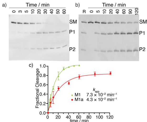
Fig. 4 Kinetics of MazF-mediated cleavage of native and 125 I modified RNA substrates ( M1 and M1a , respectively). (a) MazF-mediated cleavage of M1 . (b) MazF-mediated cleavage reaction of M1a . (c) Kinetic profiles of MazF-mediated cleavage reactions of M1 (green), M1a (red). Gels were stained by 1 × SYBR gold solution for 30 min. Lanes R correspond to native reaction indicating the cleavage site of M1a strand. Reactions were done in triplicates and a representative gel is shown per experiment. Error bars indicate SD.
