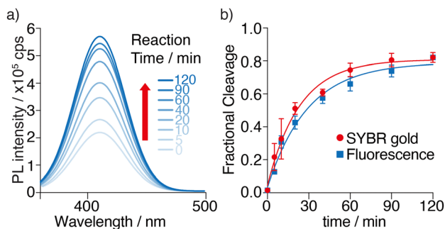
Fig. 5 MazF-mediated cleavage reaction of substrate M1a monitored by fluorescence as function of time. (a) Deconvolution of emission spectra of cleavage reaction of 125 I substrate M1a . Excitation wavelength was 341 nm. The area of each spectrum was integrated and plotted vs. time depicting the rate of the enzymatic reaction. (b) Cleavage of M1a by MazF at various time points monitored by fluorescence (blue) and SYBR gold (red). Reactions were done in triplicates and a representative deconvoluted emission spectrum is shown. Error bars indicate SD.
