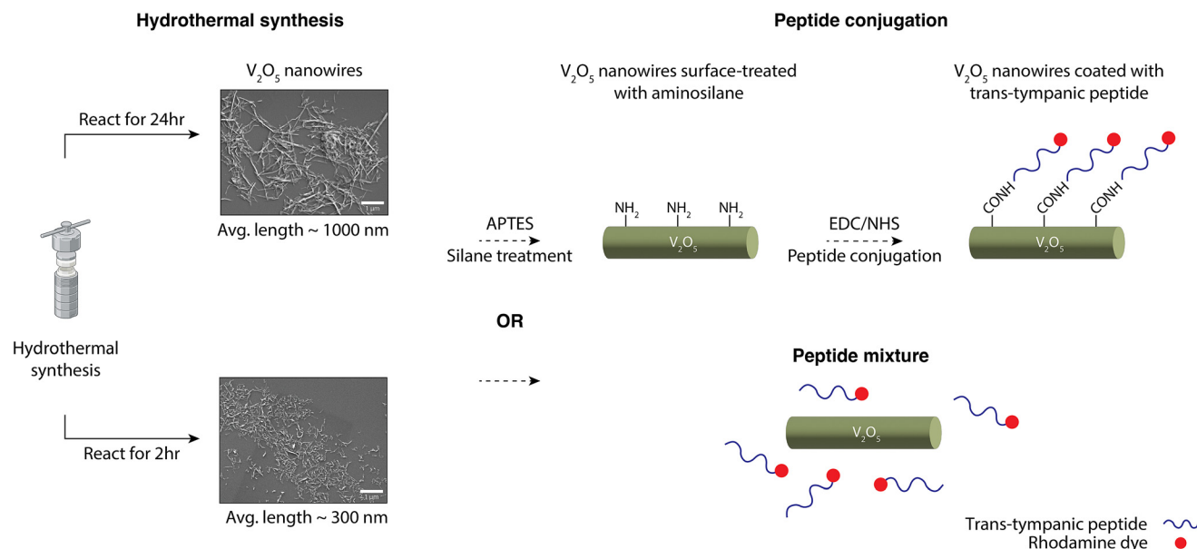
Scheme 1 An illustration showing the overall workflow of the hydrothermal synthesis of V 2 O 5 nanowires followed by mixing with peptide or peptide conjugation. During the hydrothermal synthesis step, the autoclave reaction time is tuned to regulate the average (avg.) length of the nanowires produced. The resulting nanowires are surface-modified with the TMT3 trans-tympanic peptide or mixed with the peptide. During the peptide conjugation step, the nanowires were first treated with (3-aminopropyl)triethoxysilane (APTES) to introduce amino groups onto the surface of nanowires, and then reacted with TMT3 peptide tagged with a rhodamine dye using 1-ethyl-3-(3-dimethylaminopropyl) carbodiimide (EDC) and N -hydroxysuccinimide (NHS) chemistry. Illustration partially generated with Biorender.
