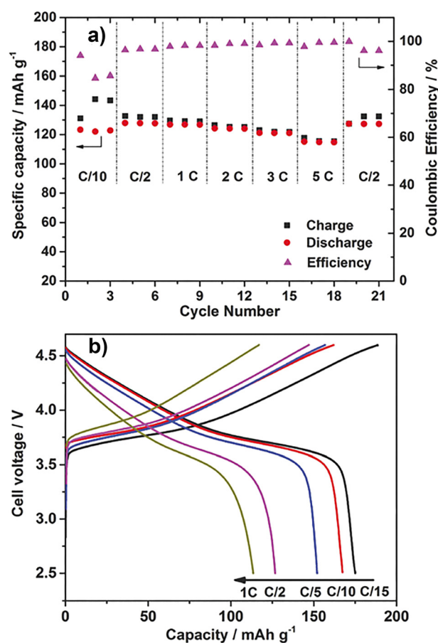
Fig. 10 Electrochemical measurements of 40 wt% \text{Li}_{0.1}\text{Ni}_{0.9}\text{b}/\text{PVDF} composites. (a) Specific capacities and coulombic efficiencies of Li/LiFePO 4 cells at different current rates, ranging from C/10 to 5C, 50 ^{\circ}\text{C} . (b) Charge-discharge curves of the Li/LiCo 1/3 Ni 1/3 Mn 1/3 O 2 cell using 40 wt% \text{Li}_{0.1}\text{Ni}_{0.9}\text{b}/\text{PVDF} composites (cut-off voltage 2.5–4.6 V), 50 ^{\circ}\text{C} . (Figure partly modified from the original one.) Reprinted from ref. 94 with permission.
