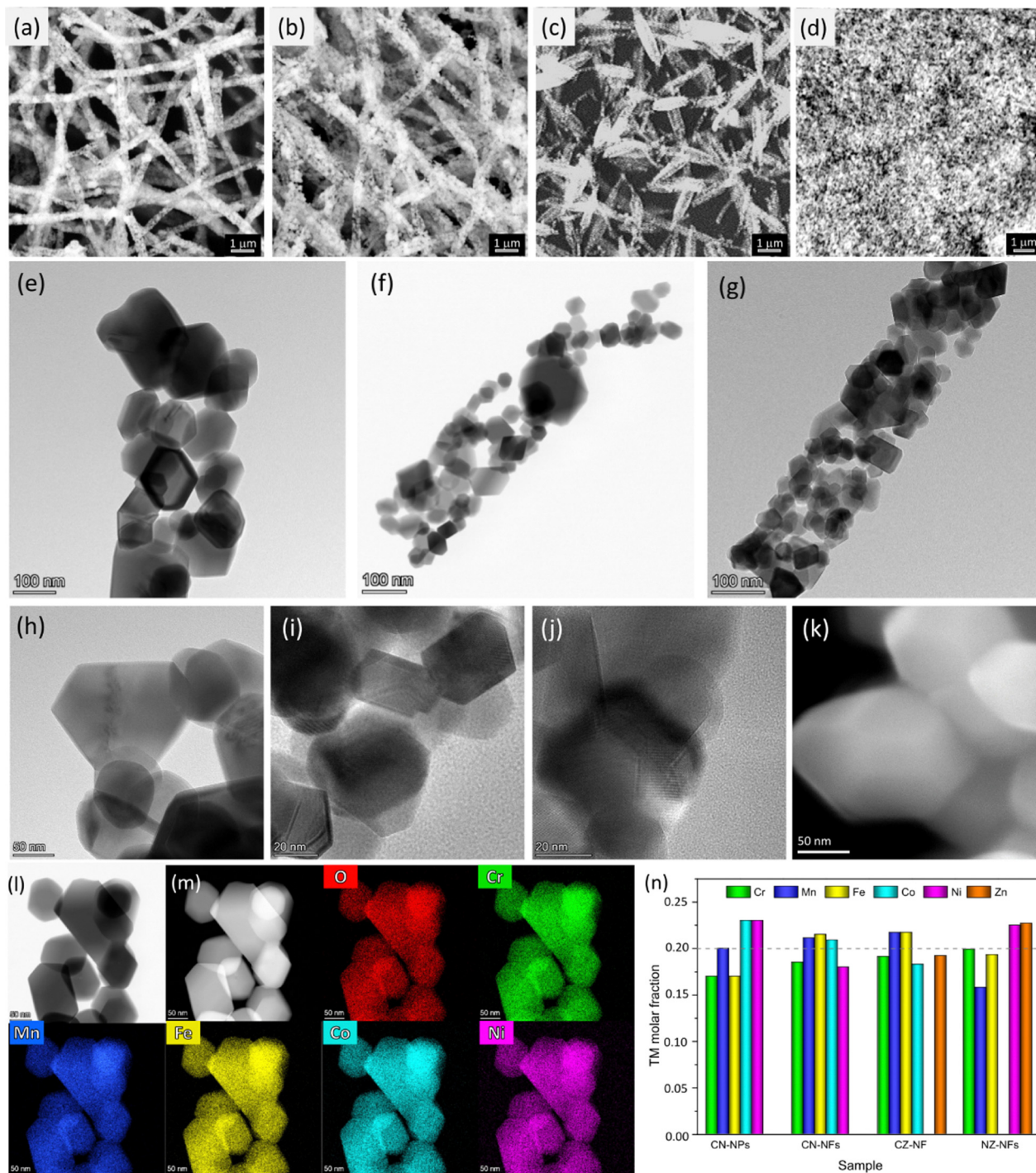
Fig. 1 Results of the SEM and HRTEM/STEM/EDX analyses on (a, e, h, k and l) CN-NFs, (b, f and g) CZ-NFs, (c, g and j) NZ-NFs and (d and k) CN-NPs. (a–d and k) SEM images, (e–j) HRTEM images; (l and m) STEM/EDX elemental maps of CN-NFs and (n) molar fraction of the TMs.
