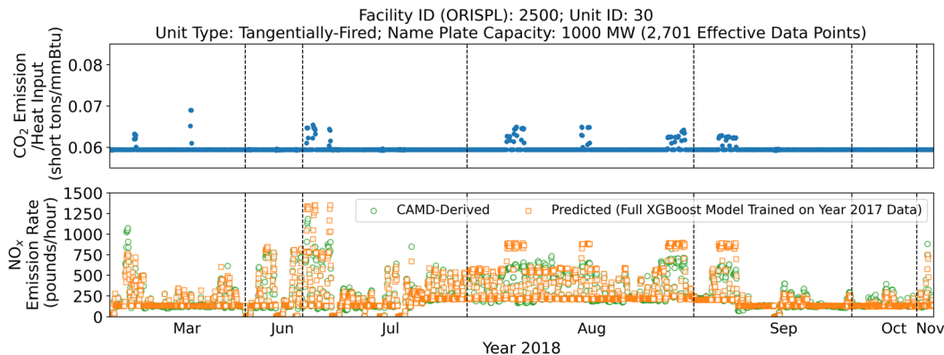
Fig. 8 The ratios between CO 2 emissions and heat input (upper), and CAMD-derived versus predicted NO x emission rates (bottom, R^2 = 0.88 ) from Unit 30 of the Ravenswood Generating Station facility in Long Island City, NY (Facility ID: 2500) in 2018, with NO x emission rates of about 160 data points over-predicted in June, July, August and September corresponded with the over-prediction zone shown in the left scatter plot in Fig. 5a.
