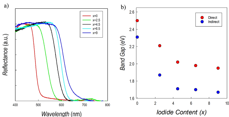
Fig. 10 (a) Reflectance spectra and (b) trend of the band gaps of the \text{Cs}_3\text{Sb}_2\text{Br}_{9-x}\text{I}_x solid solution.
