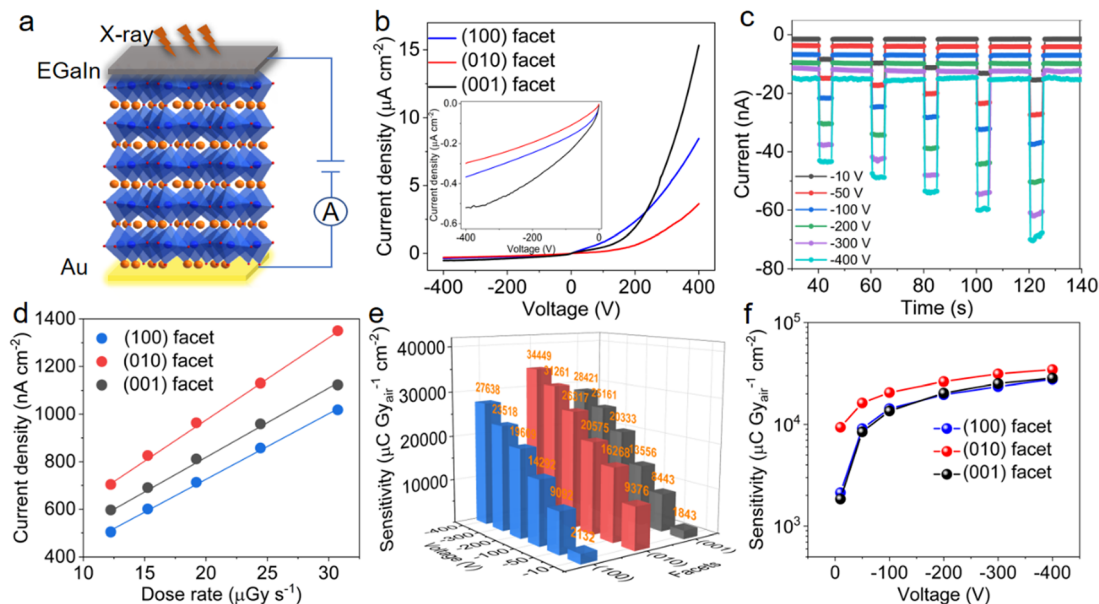
Fig. 4 (a) Schematic diagram of the CsPbBr 3 detector structure. (b) J–V curves in dark from –400 V to 400 V. The inset shows the enlarged details from –400 V to 0 V. (c) Temporal X-ray responses of the device based on the (010) wafer under voltages from –10 V to –400 V. (d) Photocurrent response via dose rates at –400 V and (e and f) X-ray sensitivities of the (100), (010), and (001) wafers under different voltages.
