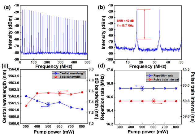
Fig. 4 Performance of the mode-locking laser based on the CsCu 2 I 3 -SA. (a) Recorded RF with a wide span. (b) Narrowband RF Spectrum. (c) Central wavelength and 3 dB bandwidth and (d) repetition rate and pulse train interval as a function of pump power.
