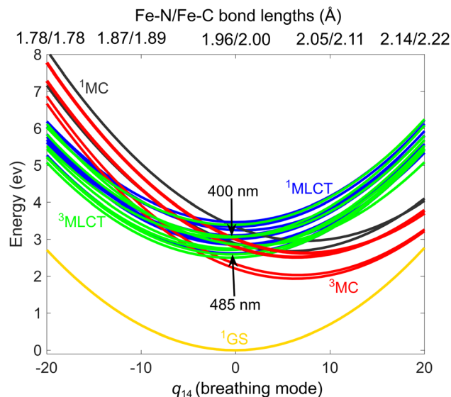
Fig. 2 Diabatic LVC-DFT/TD-DFT ground and excited-state potentials of [\text{Fe}(\text{bmip})_2]^{2+} along the breathing normal mode \nu_{14} , expressed in the dimensionless mass-frequency scaled normal mode coordinate q_{14} ; the corresponding Fe–N/Fe–C bond lengths are also shown (top axis).
