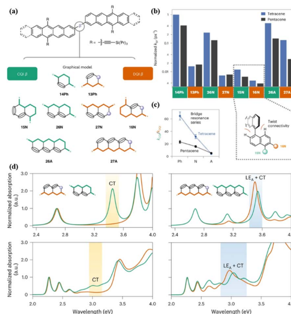
Fig. 9 (a) Bridged tetracene and pentacene dimers (top), where \beta = 14\text{Ph} ( 17 ), 13\text{Ph} ( 16 ), 15\text{N} ( 19 ), 26\text{N} ( 20 ), 27\text{N} ( 21 ), 16\text{N} ( 22 ), 26\text{A} ( 23 ) and 27\text{A} ( 24 ). (b) Comparison of SF rates (normalized to the largest k_{\text{SF}} ) across all Ph, N and A bridges in this work. Inset: chromophores attached to the 1 and/or 5 positions and the 2, 6 or 7 positions of naphthalene. (c) Changes in the CQI and DQI SF rate constants as the bridge length increases. (d) Calculated (top) and experimental (bottom) normalized absorption spectra for naphthalene-bridged tetracene dimer (left) and anthracene-bridged tetracene dimer (right). Green traces correspond to a CQI bridge (26N or 26A) and orange traces correspond to a DQI bridge (27N or 27A). The calculations assume a planar conformation. The inclusion of intermonomer rotation decreases the intensity of the CT absorption, but the absorption energy is largely unaffected. Reproduced with permission. 84 Copyright 2022, Nature.
