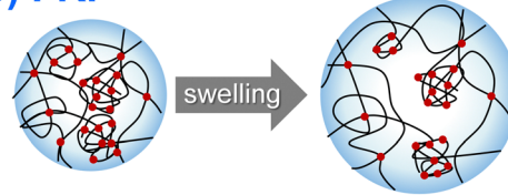
As-prepared gel
