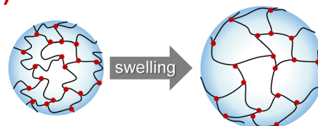
As-prepared gel
