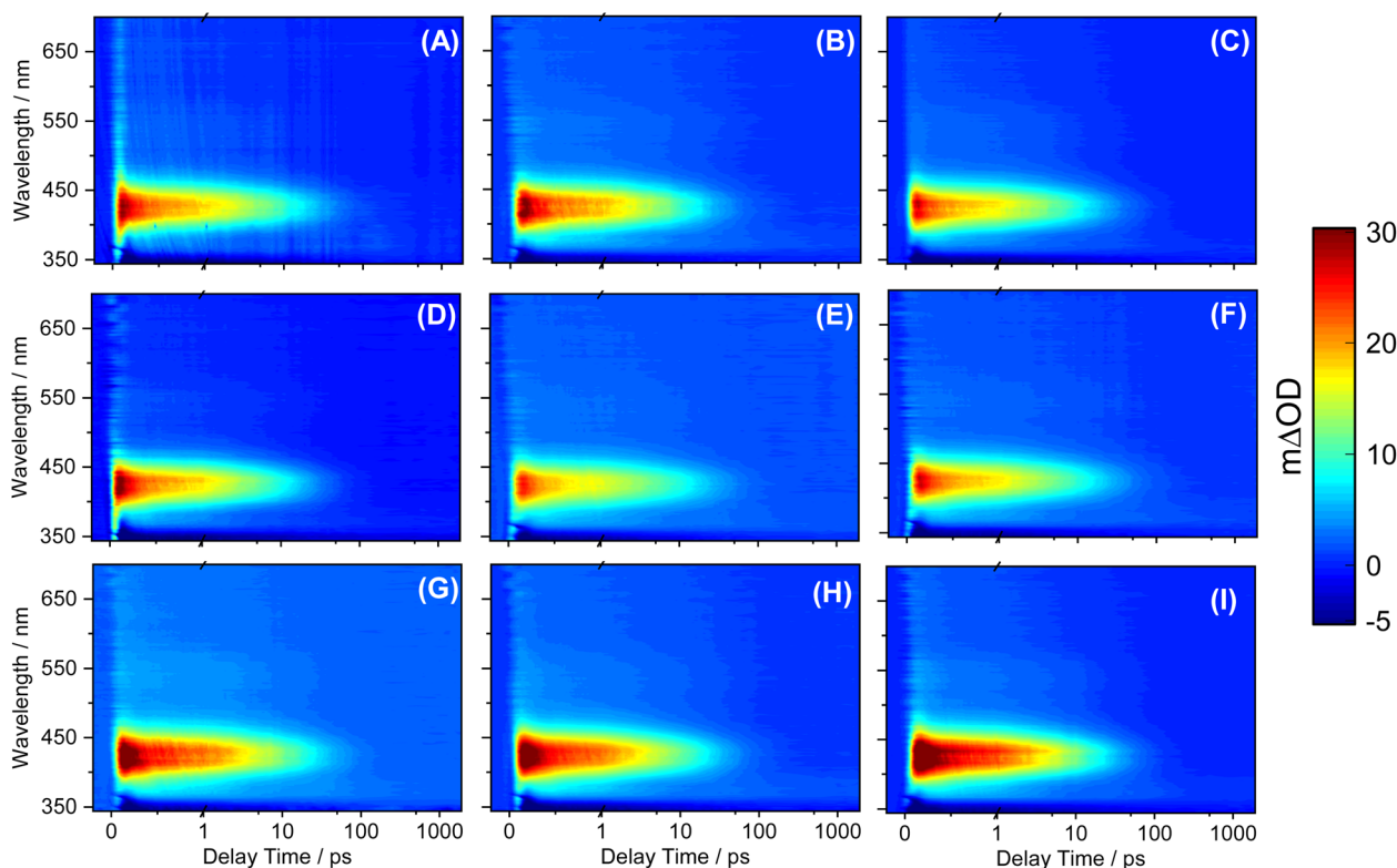
Fig. 4 TEA spectra in caprylic capric triglyceride bulk solution for (A) SM, (B) DESM, (C) DBSM (D) DOSM, (E) DSLM, (F) DCSM, (G) DGSM, (H) DFSM, and (I) DOleySM in the form of a false colour heat map indicating change in optical density ( \Delta OD ). In all cases, the delay time is presented on a linear plot until 1 ps and then as a logarithmic scale between 1 ps and 2 ns.
