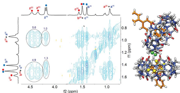
Fig. 3 1 H– 1 H NOESY spectrum of a 1:1 mixture of complex CB[7]·1 and putative aggregate (CB[7]·1) 3 Na. The correlations between adamantyl signals H a and H b with equatorial methylenes H x at the CB[7] portals are highlighted. Section of an optimized structure of putative complex (CB[7]·1) 3 Na, with interacting hydrogens H x highlighted in green, and H a and H b in yellow.
