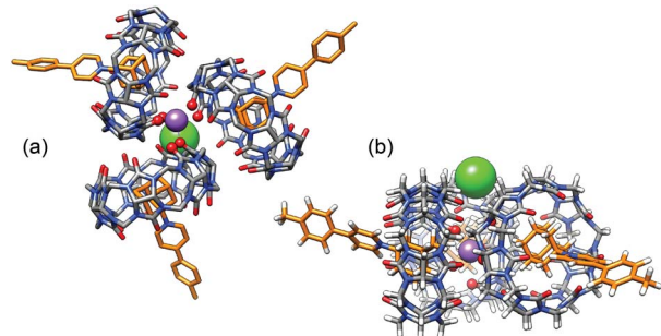
Fig. 6 (a) "Top" and (b) "side" views of GFN2-xTB-optimized 27–29 sodium-secured trimer (CB[7] \cdot 1)_3 M-X in conjunction with the ALPB solvation model for DMSO. 30 The sodium cation is deeply nested between the CB[7] carbonylated portals and the chloride anion is perched into a shallow cavity between pseudoequatorial and pseudoaxial methylene groups. Hydrogen atoms omitted for clarity in the top view.
