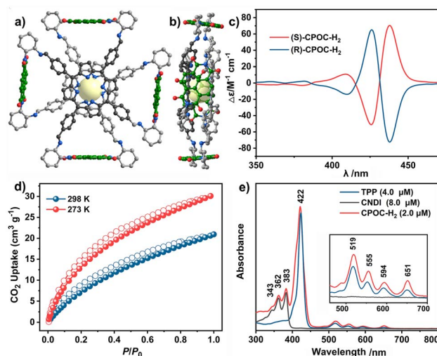
Fig. 1 Molecular structure of ( R )-CPOC- \text{H}_2 optimized by the DFT method in top (a) and side (b) view, respectively (carbon (except carbon from NDI): grey, nitrogen: blue, oxygen: red, central yellow ball represents void). (c) Circular dichroism spectra of ( R )-CPOC- \text{H}_2 (blue) and ( S )-CPOC- \text{H}_2 (red) in \text{CHCl}_3 . (d) \text{CO}_2 adsorption (solid) and desorption (hollow) curves of CPOC- \text{H}_2 at 298 K (blue) and 273 K (red). (e) Comparison of the UV-vis spectra of CPOC- \text{H}_2 and the corresponding monomeric references in \text{CHCl}_3 (inset: the enlarged spectrum from 460 to 700 nm).
