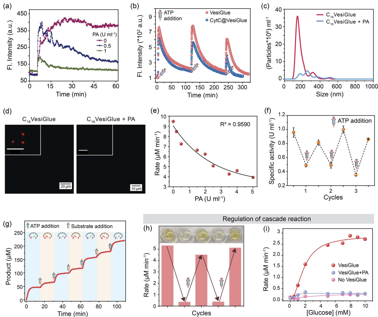
Fig. 6 Temporal control of enzyme activity and biocatalytic cascades. (a) Time-dependent fluorescence of DPH dye at 428 nm following the addition of ATP to C_{16} Gua (1 : 3) and DPH in the presence of different concentrations of potato apyrase. (b) Fluorescence Intensity at 428 nm following three repetitive additions of ATP to a system forming Vesiglu (pink) and CytC@Vesiglu (blue) in the presence of DPH and PA (1 U mL -1 ). (c) NTA measurement of Vesiglu in the presence (blue) and absence (red) of apyrase (1 U mL -1 ) where the area under the graph represents the total number of particles per mL. The particle number and uniformity decrease upon PA addition. (d) Confocal images of Nile red (NR) entrapped assembly in the absence and presence of PA (1 U mL -1 ), disruption of Vesiglu upon PA treatment releases NR leading to the disappearance of red fluorescence. The scale bar of insets is 5 \mu m. (e) The rate of biocatalytic oxidation by Vesiglu-templated CytC is modulated by the PA concentration. The black line represents exponential decay fitting to guide the eye. (f) Normalized specific activity of Vesiglu-templated CytC measured by the catalyzed oxidation of pyrogallol ( n = 3 technical replicates, mean \pm SD). Temporal regulation of CytC activity was achieved through oscillation of the ATP concentration by the presence of PA and the addition of ATP when the vesicular assemblies are disrupted at 30 min. (g) Time-dependent UV-vis traces at 420 nm (corresponding to purpurogallin formation) with time in the presence of PA. The ATP concentration leads to a higher initial rate of reaction, while the subsequent addition of pyrogallol substrate shows a much slower increase in rate due to free CytC. E and F on the clock represent empty and full ATP levels, respectively. (h) Control of the GOx/CytC/ C_{16} Vesiglu cascade reaction via ATP-Apyrase feedback control. The image shows the color change upon product formation in the corresponding microwell. (i) Rate of purpurogallin formation in the presence of varying initial substrate (glucose) concentration (0–10 mM). The decrease in the rate of cascade reaction in the presence of PA or without the Vesiglu is independent of the increasing glucose concentration. The lines represent the non-linear fitting to guide the eye.
