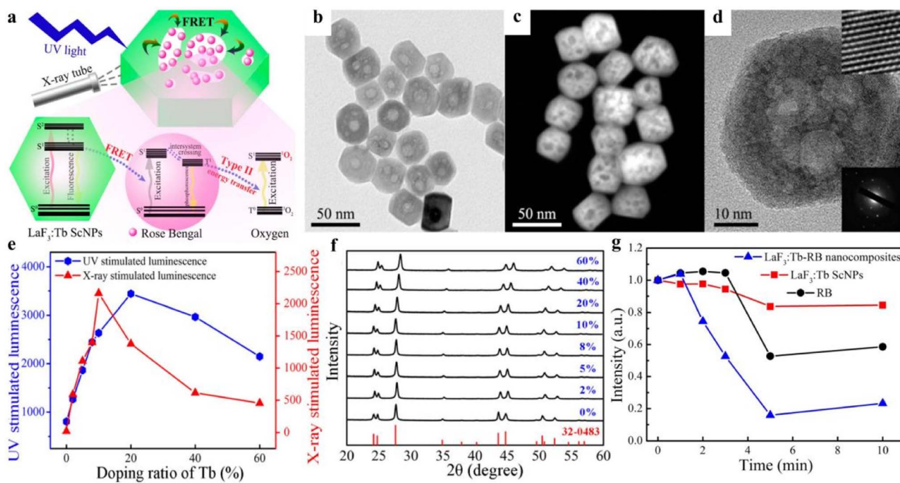
Fig. 5 (a) Schematic diagram of the structure of mesoporous LaF 3 :Tb-RB nanocomposites and their application in PDT; (b) TEM images of mesoporous LaF 3 :Tb nanoparticles, (c) SEM images; (d) HR-TEM images and SAED images; (e) UV and X-ray excitation of LaF 3 :Tb nanoparticles with different concentrations of Tb 3+ doped luminescence intensity; (f) characterizations of mesoporous LaF 3 :Tb ScNPs with varied Tb 3+ doping ratio corresponding XRD patterns; (g) decrease of emission intensity of DPBF treated with LaF 3 :Tb ScNPs, RB, and LaF 3 :Tb-RB nanocomposites, respectively, after different irradiation time. 26
