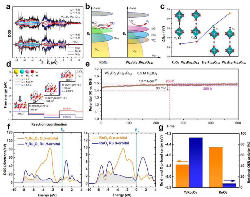
Fig. 10 (a) DOS plots of Ru 4d and O 2p states in RuO 2 and W 0.2 Er 0.1 Ru 0.7 O 2-δ-1 . (b) Schematic representation of rigid band models for RuO 2 and W 0.2 Er 0.1 Ru 0.7 O 2-δ-1 toward acidic OER. (c) The formation energy of V O at different positions. (d) Diagram of the energy barrier for W 0.2 Er 0.1 Ru 0.7 O 2-δ-1 . (e) The long-term stability (500 h) of W 0.2 Er 0.1 Ru 0.7 O 2-δ-1 nanosheets in 0.5 M H 2 SO 4 . (a–e) Reprinted with permission from ref. 104. Copyright 2020, Springer Nature. (f) Calculated PDOS plots of Ru 4d and O 2p orbitals for Y 2 Ru 2 O 7 and RuO 2 . (g) Comparison of the central energies of the overlapping bands of Ru 4d and O 2p orbital and retained current density at 1.50 V for Y 2 Ru 2 O 7 and RuO 2 , respectively. (f and g) Reprinted with permission from ref. 108. Copyright 2017, American Chemical Society.
