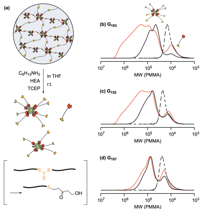
Fig. 6 (a) Degradation of POSS-crosslinked hydrogels by the aminolysis reaction and (b)–(d) SEC curves of the degradation product of the gels with various molecular weights (red line: degradation products from gels after a heating/cooling cycle, black solid line: degradation products from gels before a heating/cooling cycle, and black dotted line: prepolymers).
