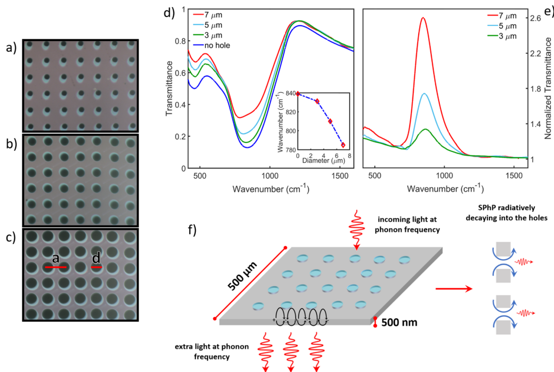
Fig. 2 Optical microscope images of the patterned Si 3 N 4 samples, with 3 μm (a), 5 μm (b) and 7 μm (c) hole diameters d , and lattice parameter a = 12 μm. (d) Shows the transmittance spectra for unpatterned and patterned samples. (e) Depicts instead the normalized transmittance, defined as the ratio between the transmittance of each patterned sample and the one of the unpatterned. (f) Sketch depicting the self-standing 500 nm thick Si 3 N 4 membrane patterned with circular holes, filled with air. The membrane side is 500 μm. This picture schematically describes the EOT phenomenon, in which the incoming light at phonon frequency excites a surface phonon polariton, indicated by black arrows, trapped at the air–membrane interface. The scattering process and the radiative decay of this mode through the holes generate extra light at phonon frequency, giving rise to the EOT phenomenon, as described, for instance, in ref. 42.
