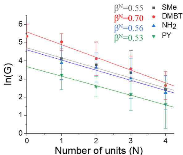
Fig. 2 Plot of the most probable experimental conductance values \ln(G) versus number of units -N- , N , from STM-BJ measurements in mesitylene.
