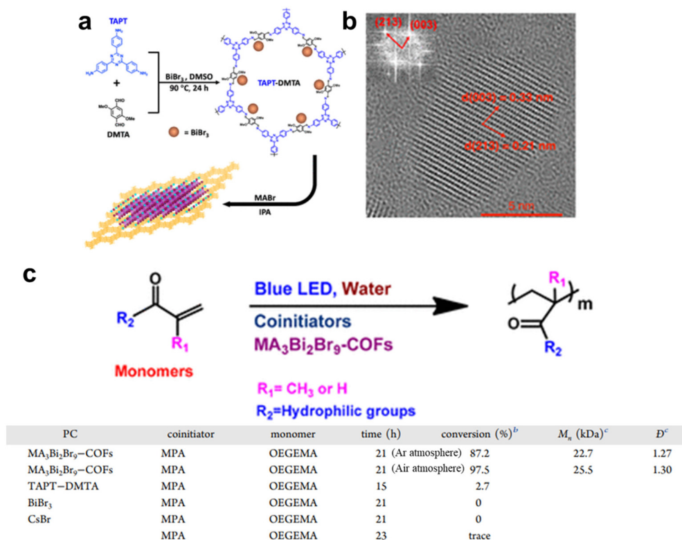
Fig. 12 (a) The in situ synthetic protocol for \text{MA}_3\text{Bi}_2\text{Br}_9 -COFs nanocomposites. (b) The HRTEM image indicating the formation of \text{MA}_3\text{Bi}_2\text{Br}_9 NCs-COFs nanocomposites; inserted graph: FFT pattern of the selected area. (c) Partial results of photoinduced polymerization reactions using \text{MA}_3\text{Bi}_2\text{Br}_9 -COFs nanocomposites in water. Reproduced with permission from ref. 135. Copyright 2022 American Chemical Society.
