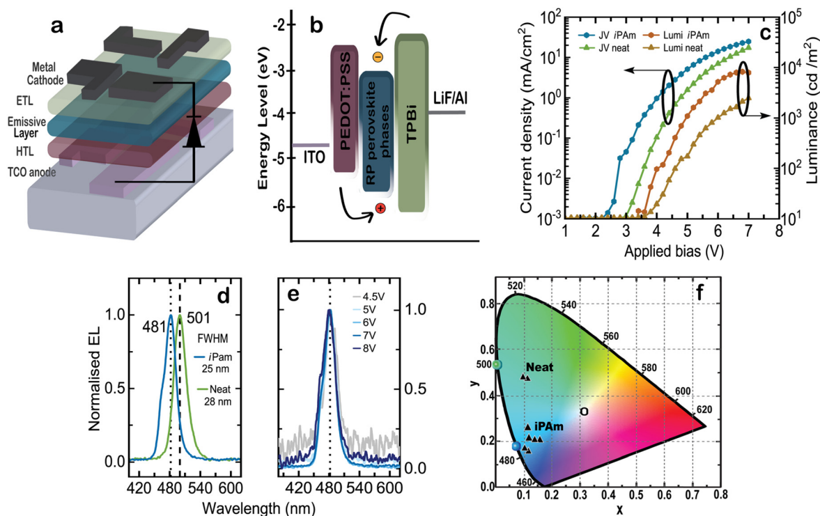
Fig. 6 (a) Schematic illustration of the structure of our PeLED and (b) energy level alignment of the materials comprising the device structure. (c) JVL curves of the champion iPA and neat devices. (d) EL spectra of iPA and neat PeLEDs recorded at an applied bias of 7 V. (e) EL spectra of blue-emitting iPA PeLED at different applied biases. (f) CIE colour coordinates of the best performing iPA and neat devices.
