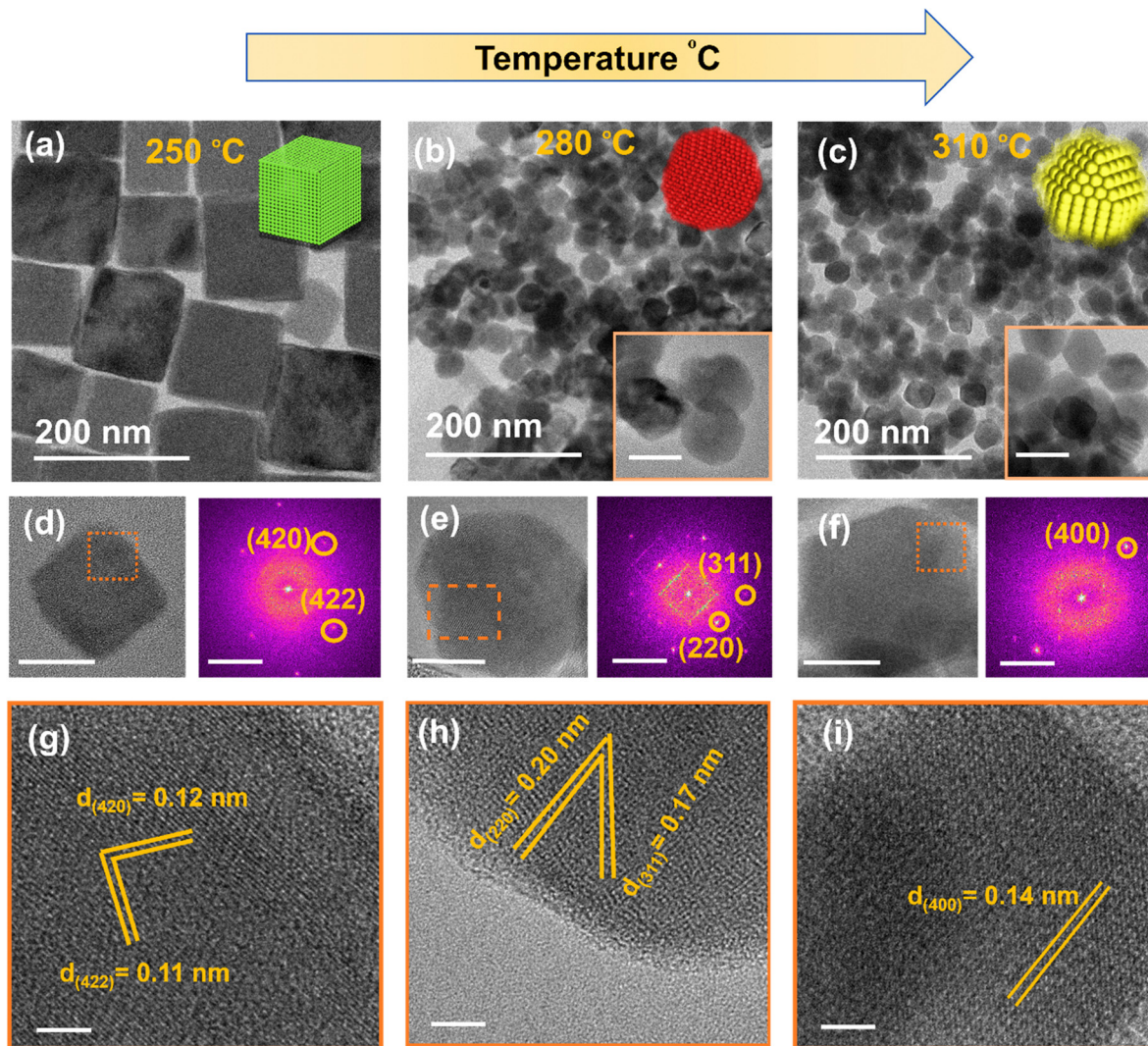
Fig. 2 (a–c) TEM images of NaSb 2 NCs formed at 250, 280 and 310 °C, respectively the scale bar in the inset images is 50 nm. (d–f) are the magnified images (scale bar is 50 nm) and FFT patterns. (g–i) magnified images of NaSb 2 NCs. The scale in panels (g–i) is 5 nm respectively.
