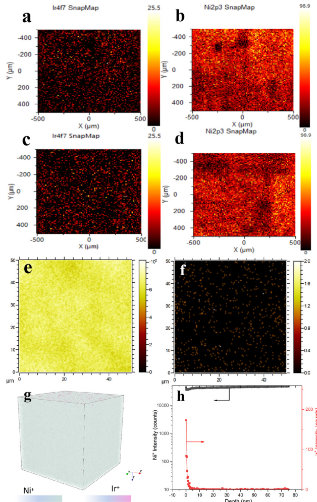
Fig. 5 Surface element mapping images from XPS spectra over fresh Ir/Ni and used Ir/Ni catalyst. The spot size was controlled at 10 \text{ \mu m} , and the scanning times were 20 for each spot. (a) Ir and (b) Ni mapping spectra over a fresh Ir/Ni sample. (c) Ir and (d) Ni mapping spectra over a used Ir/Ni sample. Abundance maps of (e) \text{Ni}^+ and (f) \text{Ir}^+ over a 50 \times 50 \text{ \mu m}^2 field of view from the Ir/Ni surface region. (g) A 3D TOF-SIMS map of the Ir signal on the Ni substrate. (h) The \text{Ni}^+ and \text{Ir}^+ signals obtained by TOF-SIMS analysis with respect to the diffusion depth.
