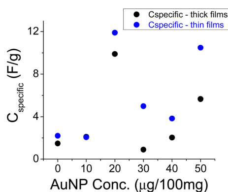
Fig. 7 Specific capacitance, C_{\text{specific}} in units of \text{F g}^{-1} from C-V data for thick and thin films with a CAB binder. The concentration of AuNPs in \mu\text{g} is referenced to the amount of AC mass in the slurry, in 100 mg. The C_{\text{specific}} value for 10 \mu\text{g} per 100 mg of AC is identical for both films. The electrolyte was 1 M \text{Na}_2\text{SO}_4 .
