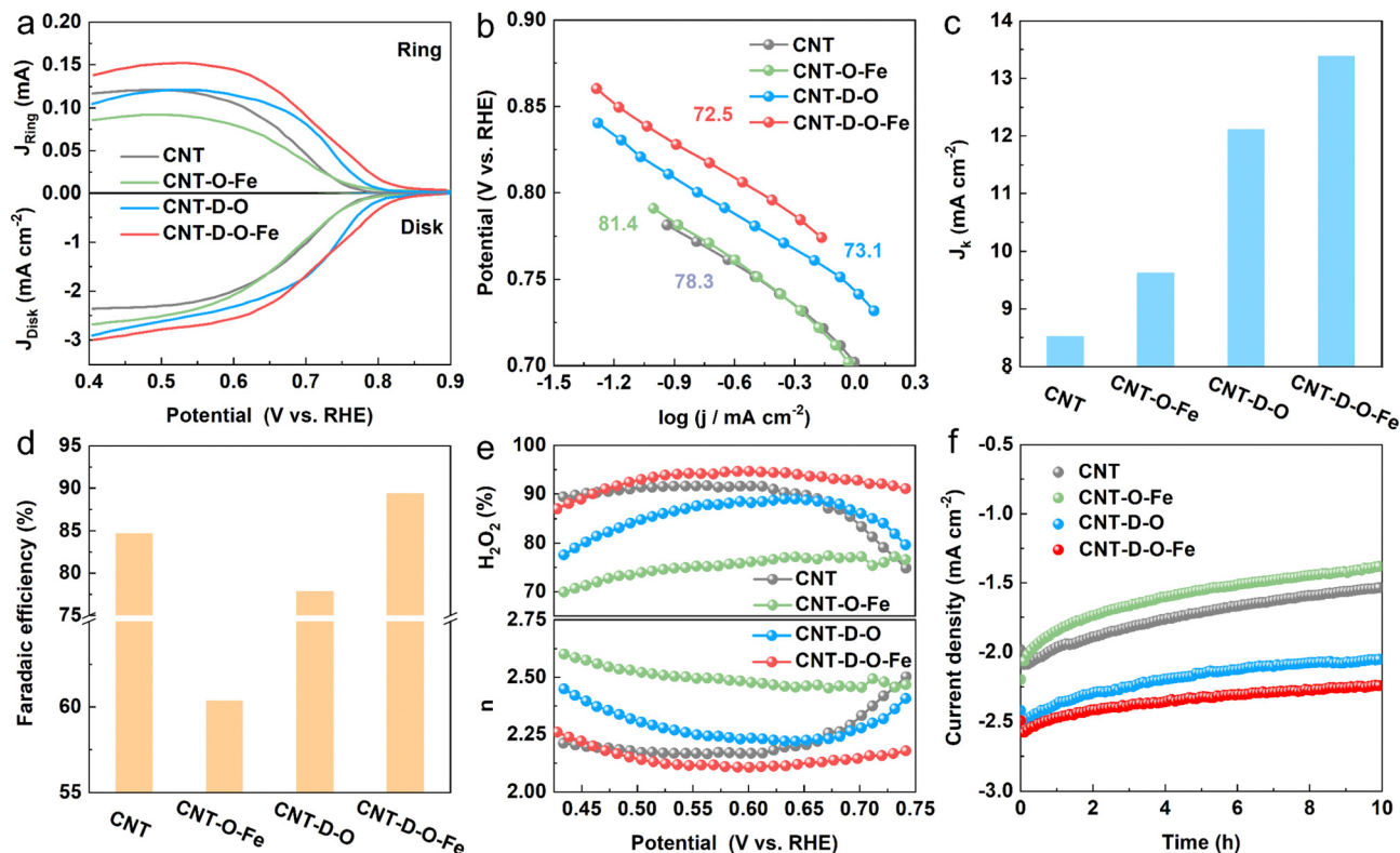
Fig. 4 (a) LSV curves (ring current and disk current density, respectively), (b) the Tafel plots of CNT, CNT-O-Fe, CNT-D-O, and CNT-D-O-Fe; (c) J_k and (d) faradaic efficiency for H 2 O 2 at 0.550 V vs. RHE, (e) electron transfer number and selectivity for H 2 O 2 ; (f) stability test of the catalytic materials at 0.550 V vs. RHE.
