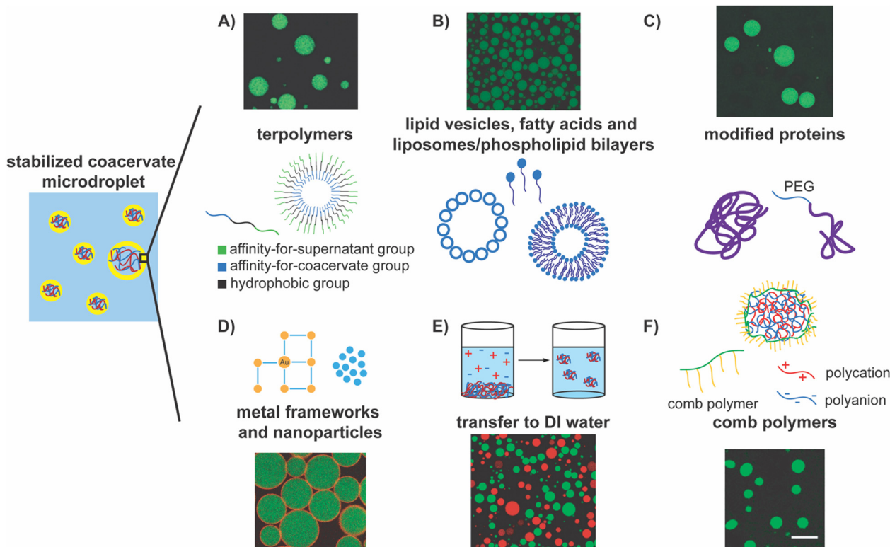
Fig. 3 Highlights of the approaches for stabilizing complex coacervate droplets. In the schematic on the left, polyanions are depicted as blue chains, polycations as red chains, the polymer-lean supernatant phase is depicted by the blue region, and the yellow region depicts the interface between the coacervate and the supernatant phases. (A) Terpolymer, or triblock copolymers, form polymersomes that stabilize the coacervate droplets. In the schematic, the green block has an affinity for the supernatant group, the blue block has an affinity for the coacervate, and black blocks is hydrophobic. The fluorescent image shows stabilization of droplets using this kind of terpolymers. 166 Reprinted with permission from Methods in Enzymology , Elsevier. (B) Different self-assemblies of lipids, including lipid vesicles, fatty acids, liposomes, and phospholipid bilayers can serve as stabilizers of coacervate droplets. The fluorescent image shows stabilization of coacervate droplets by phospholipid vesicles. 154 Reprinted (adapted) with permission from F. Pir Cakmak, A. T. Grigas and C. D. Keating, Langmuir , 2019, 35 , 7830–7840. Copyright 2019 American Chemical Society. (C) Modified proteins can serve as stabilizers for the coacervate/water interface. The fluorescent image shows stabilization of coacervate microdroplets by mPEG-modified BSA accumulated at the interface. 173 Reprinted with permission from Small , Wiley. (D) Nanoparticles and metal frameworks can assemble at the coacervate/water interface and stabilize them. The fluorescent image shows gold/PEG nanoparticle stabilization of the coacervate/water interface. 177 Copyright 2022 American Chemical Society. Available under the Creative Commons Attribution 4.0 International Public License. No modification to the material was made. (E) Transfer of coacervate droplets from supernatant phase to DI water as a method of stabilizing coacervate droplets. The fluorescent image shows stable coacervate microdroplets in DI water. 178 Copyright 2022 A. Agrawal, J. F. Douglas, M. Tirrell, and A. Karim. Available under the Creative Commons Attribution 4.0 International Public License. No modification to the material was made. (F) Comb polymer stabilization of polyelectrolyte complexes via interfacial assembly. The fluorescent image shows stable coacervate droplets. 80 Reprinted (adapted) with permission from S. Gao and S. Srivastava, ACS Macro Lett. , 2022, 11 , 902–909. Copyright 2022 American Chemical Society.
